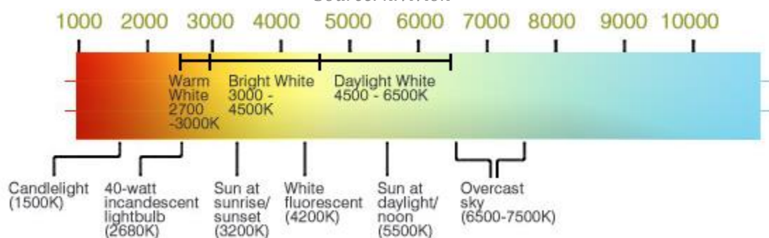
Figure 2: The Kelvin scale
